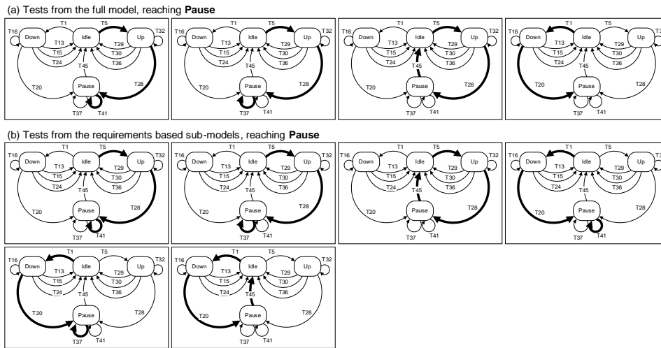
Figure 5: Comparison of test cases reaching the Pause state. (Test cases are indicated by the sequence of bold transitions in the model.)
